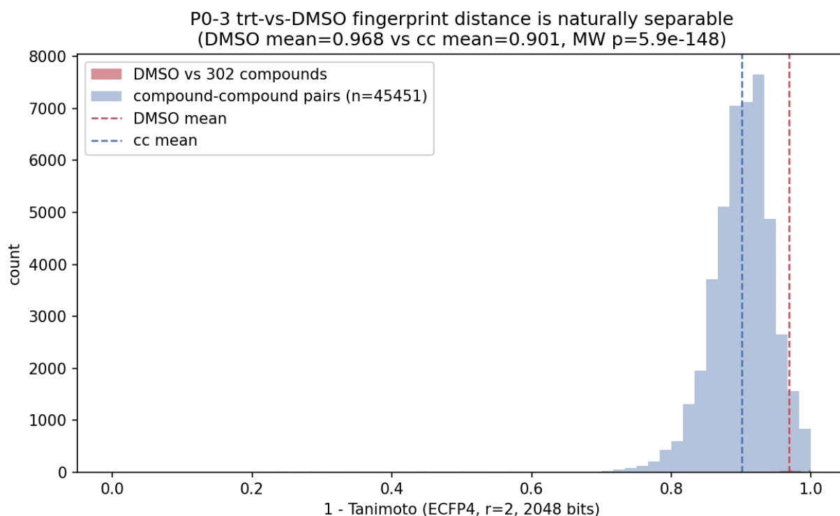
FP distance distributions
