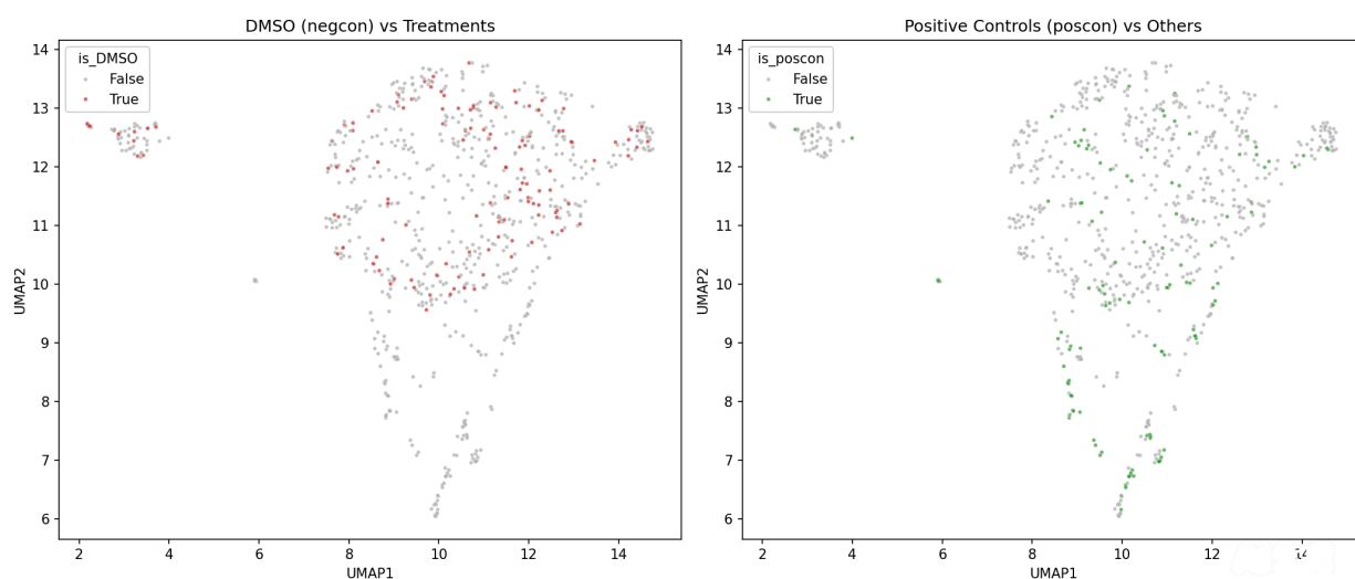
UMAP of well-level profiles
