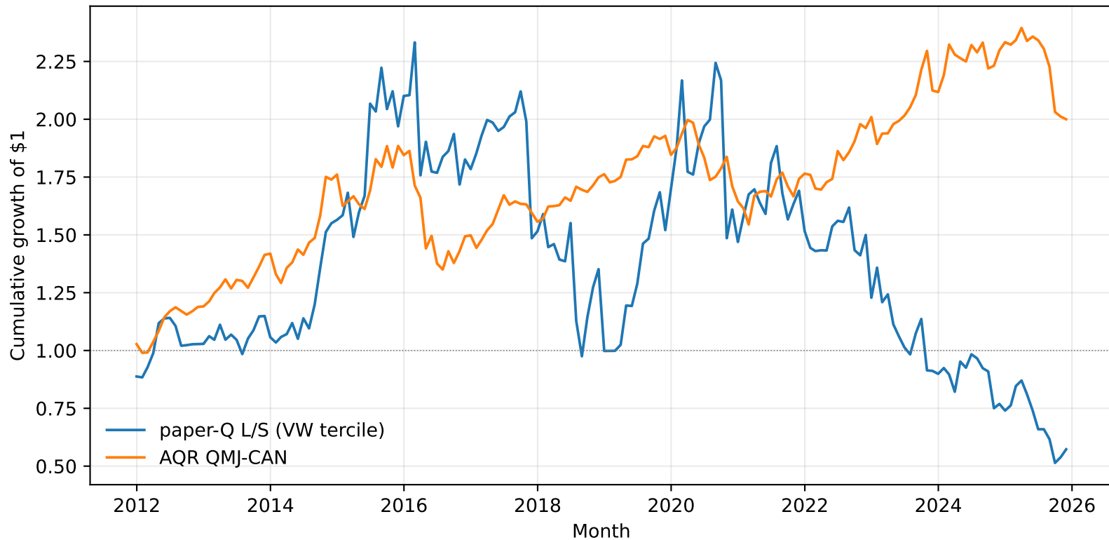
paper-Q (TSX small/mid-cap) vs AQR QMJ-Canada
