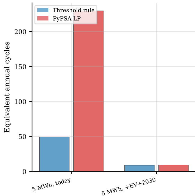
(b) Battery throughput
