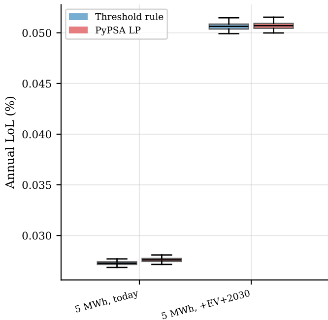
(a) Annual LoL: threshold vs PyPSA LP
