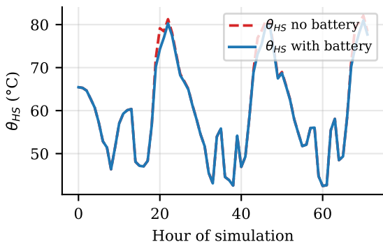
(c) Hot-spot temperature: battery shaves the EV-driven peak
