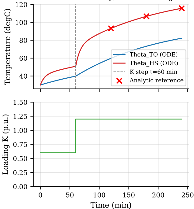
IEEE C57.91-2011 Annex G Validation K=0.6 to K=1.2 step, ambient=30 degC
