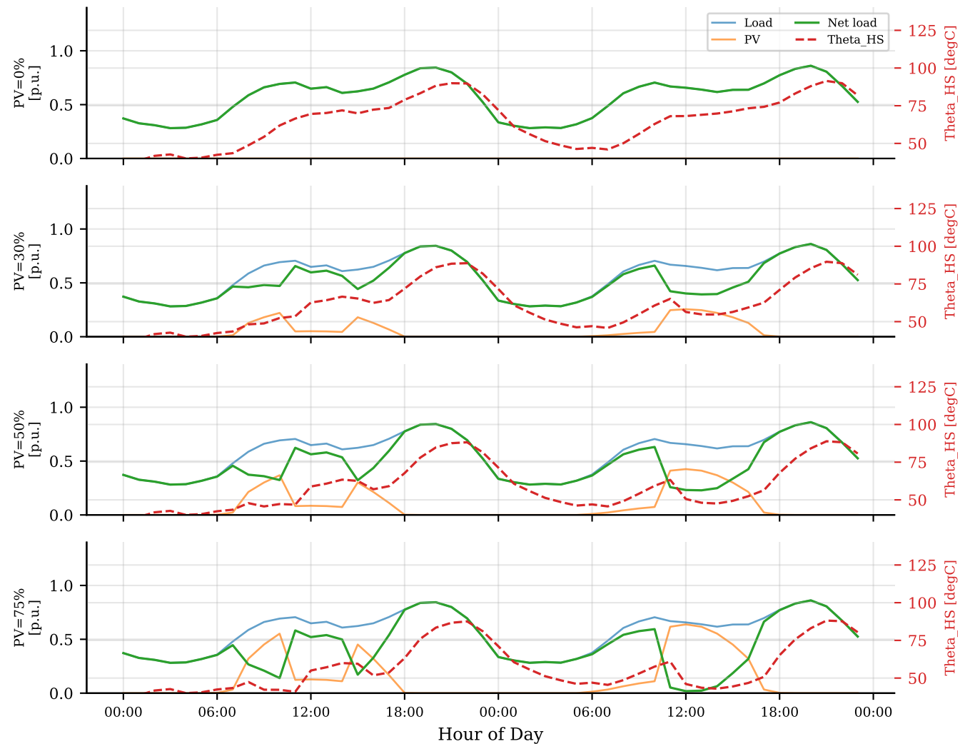
48h Load, PV, Net Load and Hot-Spot Temperature for Four PV Penetration Levels
