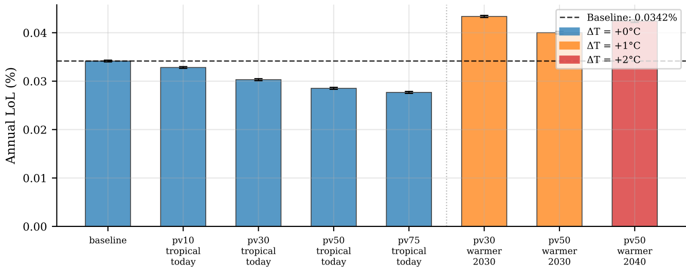
Annual Transformer Loss-of-Life: Named Scenarios (mean \pm 1\sigma , 1000 MC runs each)
