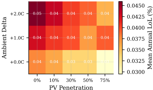
Mean Annual LoL Sensitivity (PV Penetration x Ambient Delta)
