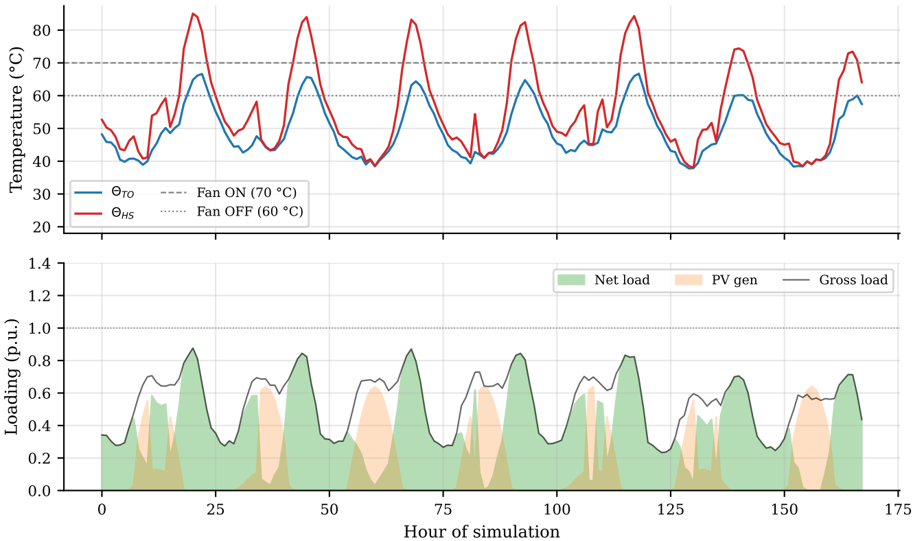
ONAN/ONAF Mode Switching — 7-day trace, PV=75%
