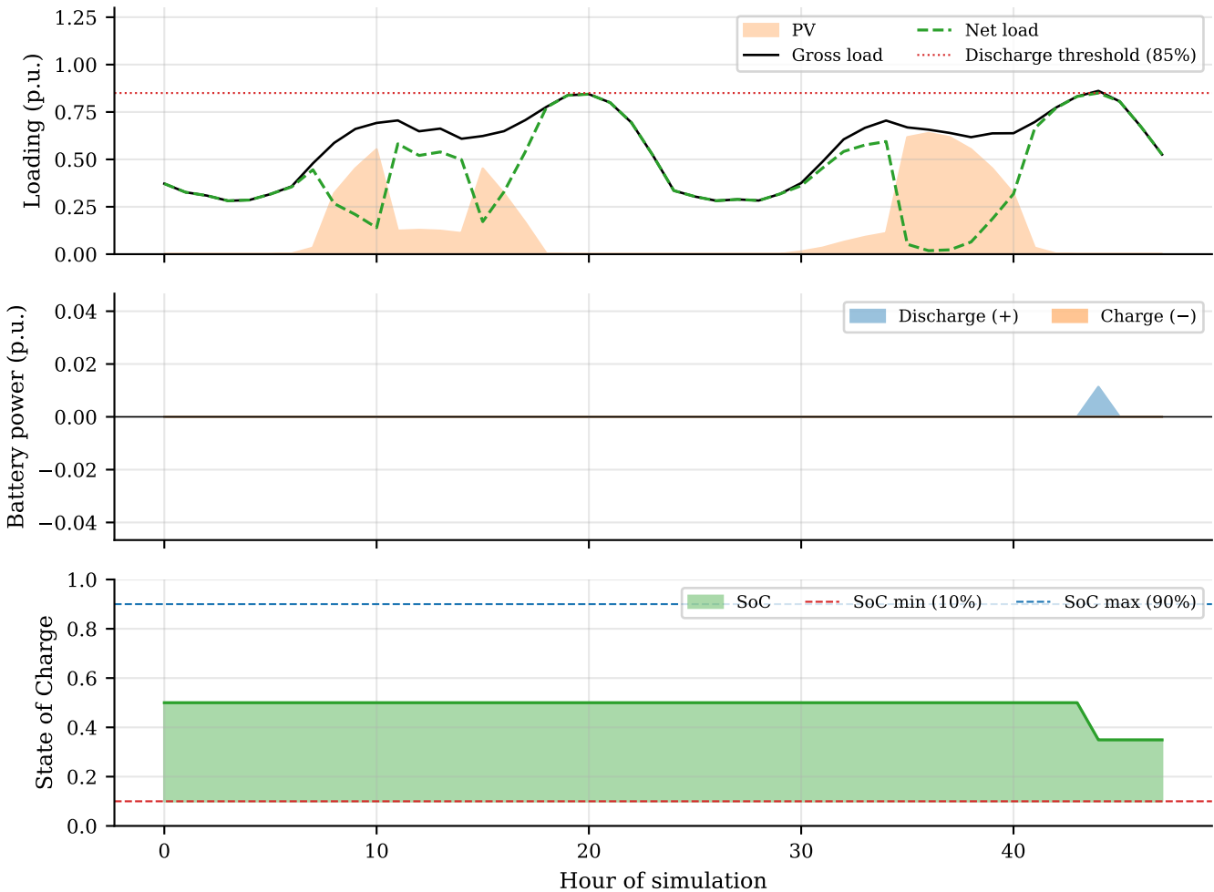
Battery Dispatch — 48 h trace, PV=75%, 5 MWh / 2 MW
