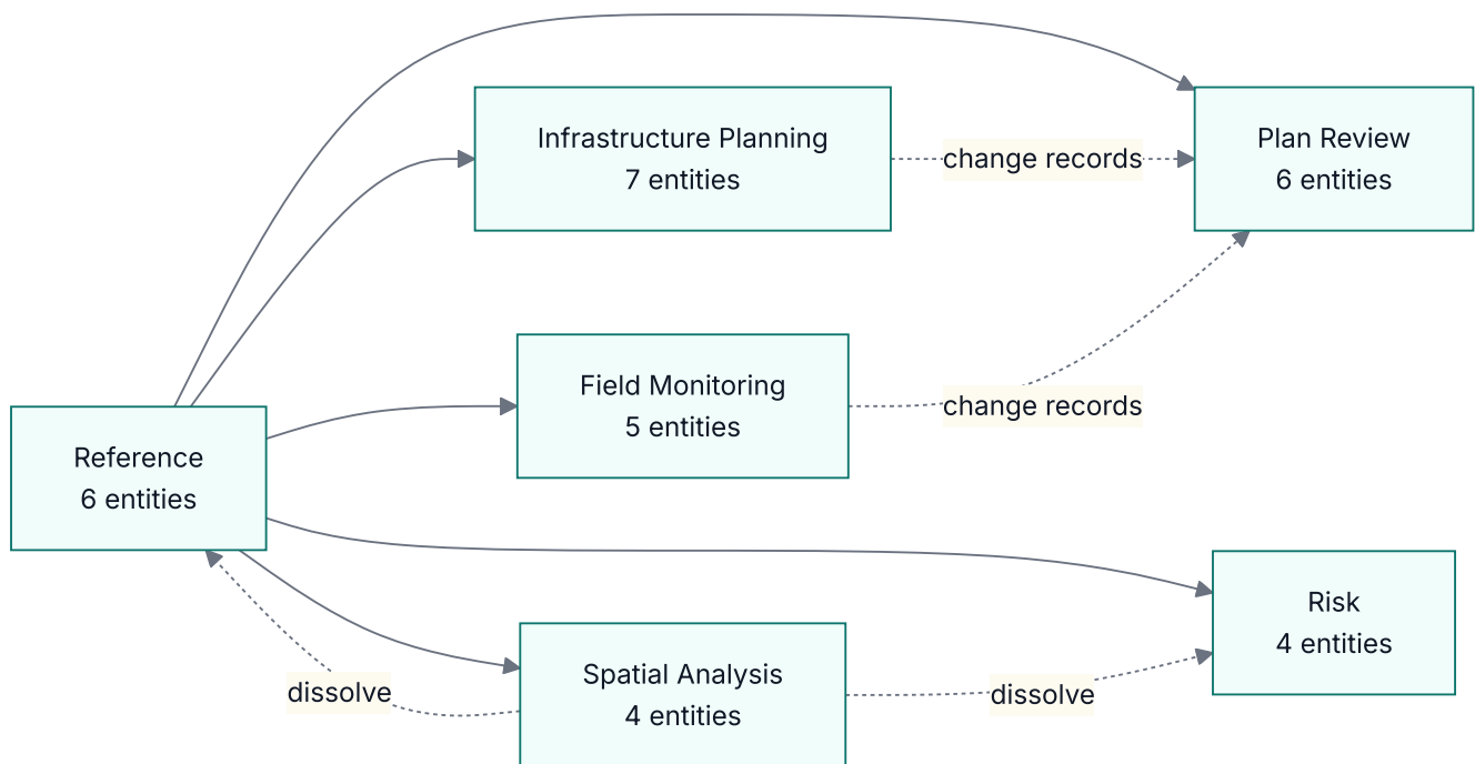
Figure 1. Contexts and their dependencies. Solid lines are foreign keys, dotted lines are data flows (dissolve during load, change records written by triggers).
