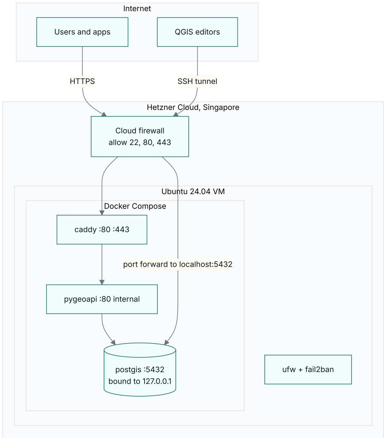
Figure 5. Production style deployment.
