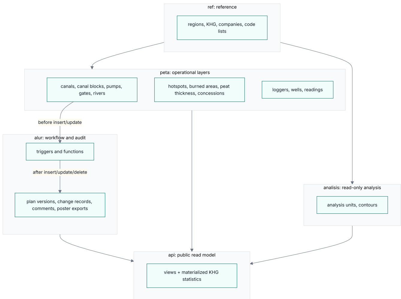
Figure 3. Database schemas and how triggers connect them.
