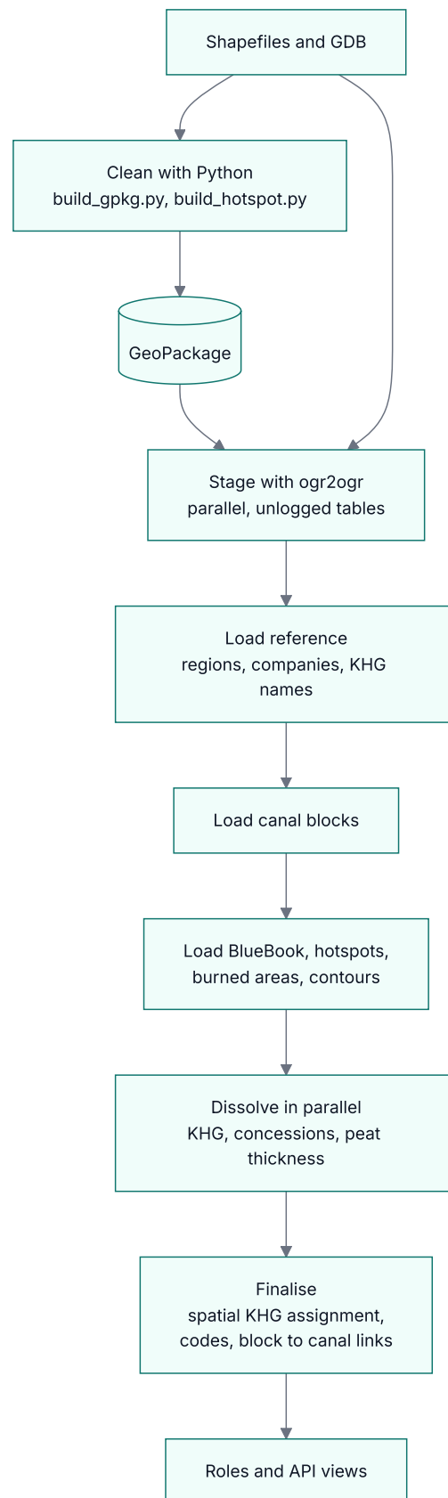
Figure 4. Build pipeline run by db/setup.sh.
