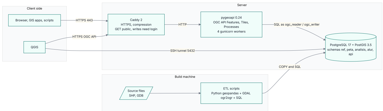
Figure 2. Containers and their connections.
