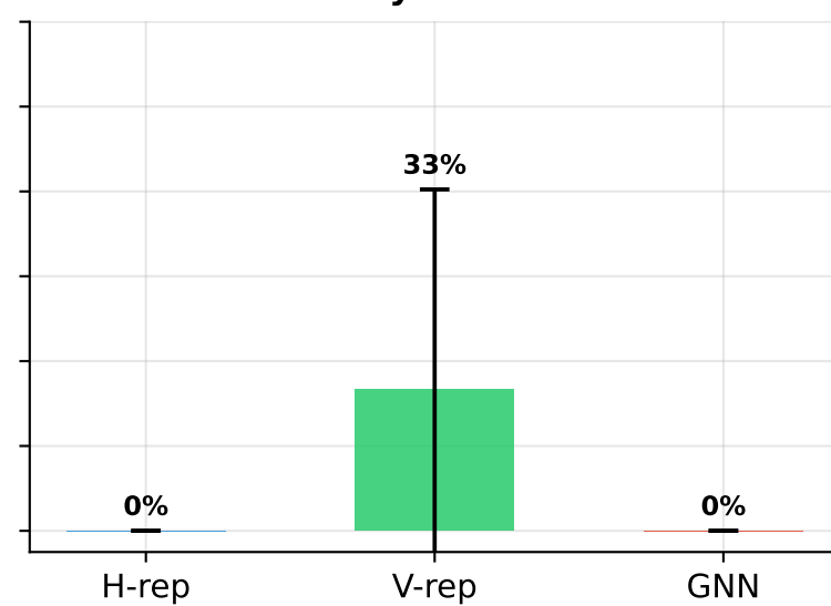
Difficulty 15 moves
