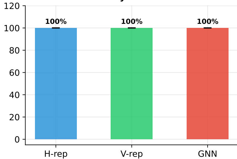
Difficulty 10 moves
