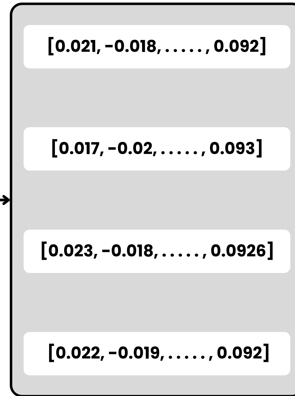
Embeddings
