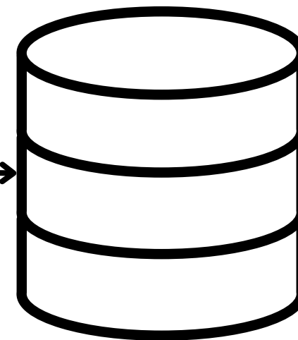
Vector Database
