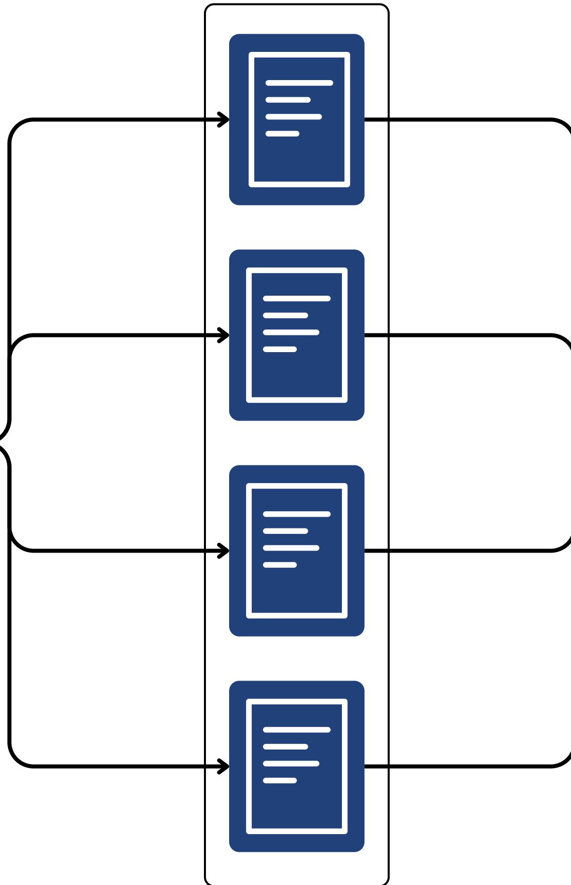
Chunks
