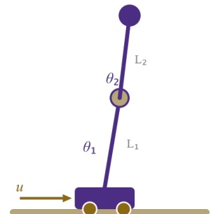
Figure 1. IDP geometry. State \mathbf{x} = [x, \theta_1, \theta_2, \dot{x}, \dot{\theta}_1, \dot{\theta}_2] . Tip height h \in [0, 1.2] m; episode ends at h <
