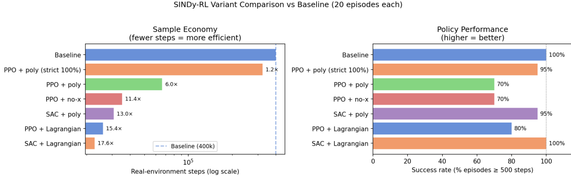
Figure 6. All SINDy-RL variants versus the 400,000-step full-order baseline (20 episodes each). Left: real-environment steps on log scale (fewer = more efficient). Right: task success rate. The “strict 100%” bar is a stress-test continuation experiment under a harder criterion (full-horizon 999 steps) that consumed 323k+ steps to reach 95% success, confirming that brute-force iteration cannot substitute for appropriate library and optimizer choices.
