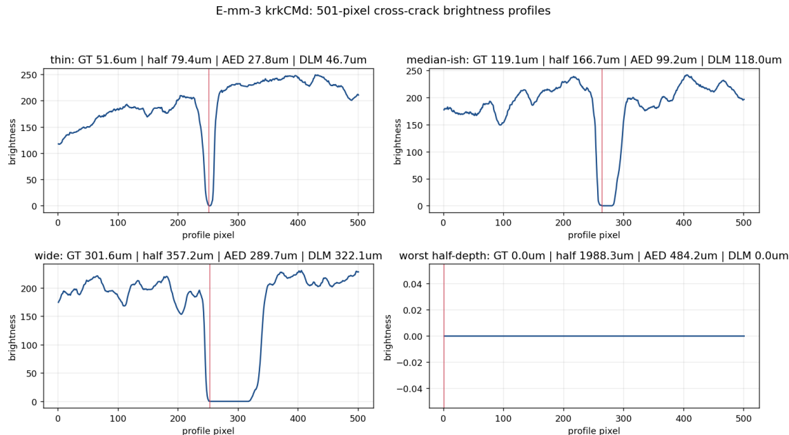
Figure 3: krkCMd cross-crack brightness profiles (501 samples, 3.97 \mu\text{m}/\text{px} ) with manual width GT—the physical ground truth behind Table 2.
