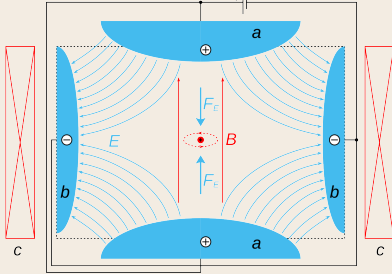
Figure 4: Schematic view of Penning trap with electric (blue) and magnetic (red) field indicated, generated by electrodes and coils respectively
