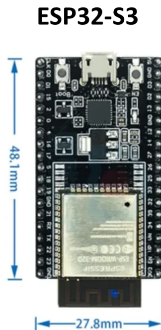
Gambar 12: Microcontroller Unit ESP32-S3
