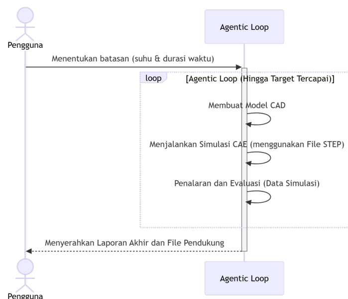
Gambar 16: Cara kerja Agentic Loop
