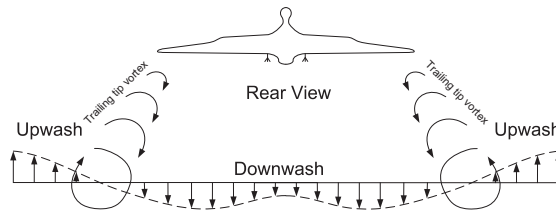
Fig. 2. Regions of upwash and downwash created by trailing vortices.
