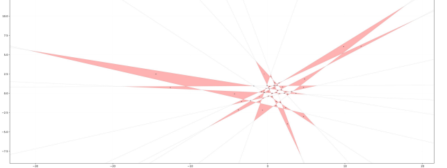
Figure 1: Geometric configuration of the K(14) = 54 solution. This configuration was isolated using the Vectorial Taboo Search and validated via CPU-based intersection analysis.
