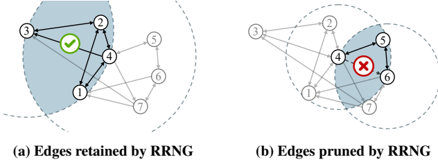
Figure 2: Illustration of the RRNG pruning strategy
