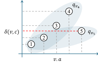
Figure 5: Illustration of entry node set generation
