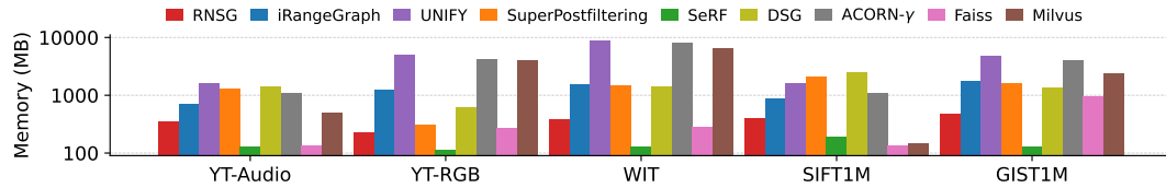
Figure 8: Index size of different methods on all datasets
