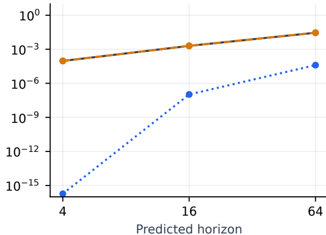
Entropy simplex
