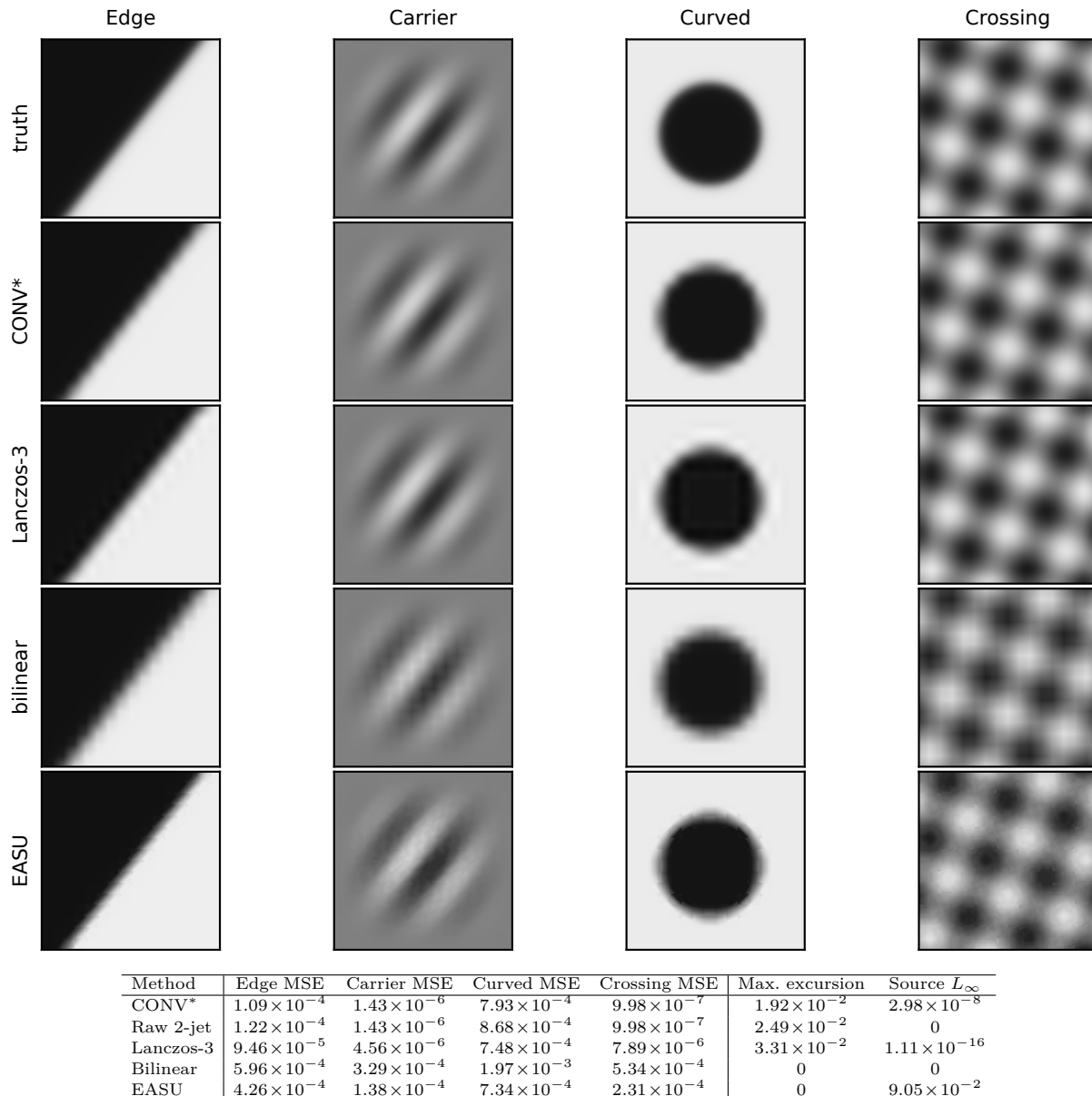
Fig. 5. Technical synthetic fields and their local comparison grid. Images use a dense endpoint-aligned query lattice and one common [0, 1] display scale; the table reports unquantized binary64 values at target side 33 against direct analytic evaluation.
