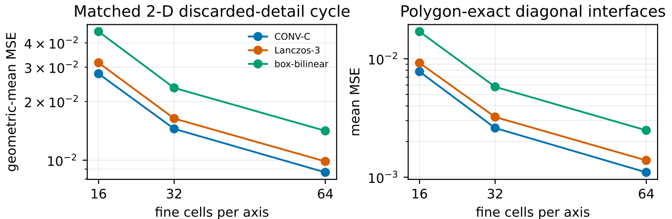
Fig. 3. Conservative zero-detail transform ablation. Left: geometric-mean MSE over all 14 two-dimensional cases at each size. Right: mean MSE over the eight polygonal diagonal interfaces. Each curve uses its method’s declared analysis and synthesis.
