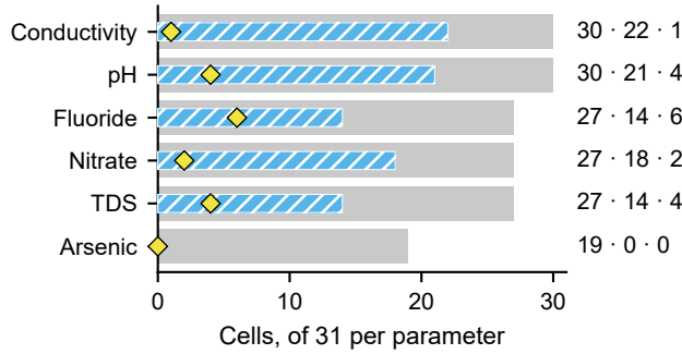
A Record support by parameter
