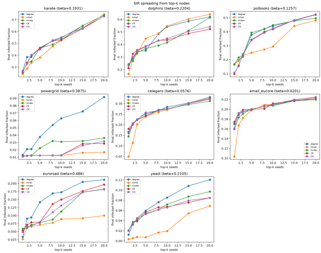
Figure 4. SIR spreading from top-k seeds ( \beta = 1.5\beta_c , \gamma = 1 , 200 \times 100 steps, seed 42). Degree dominates; CIC is close on small social networks.
