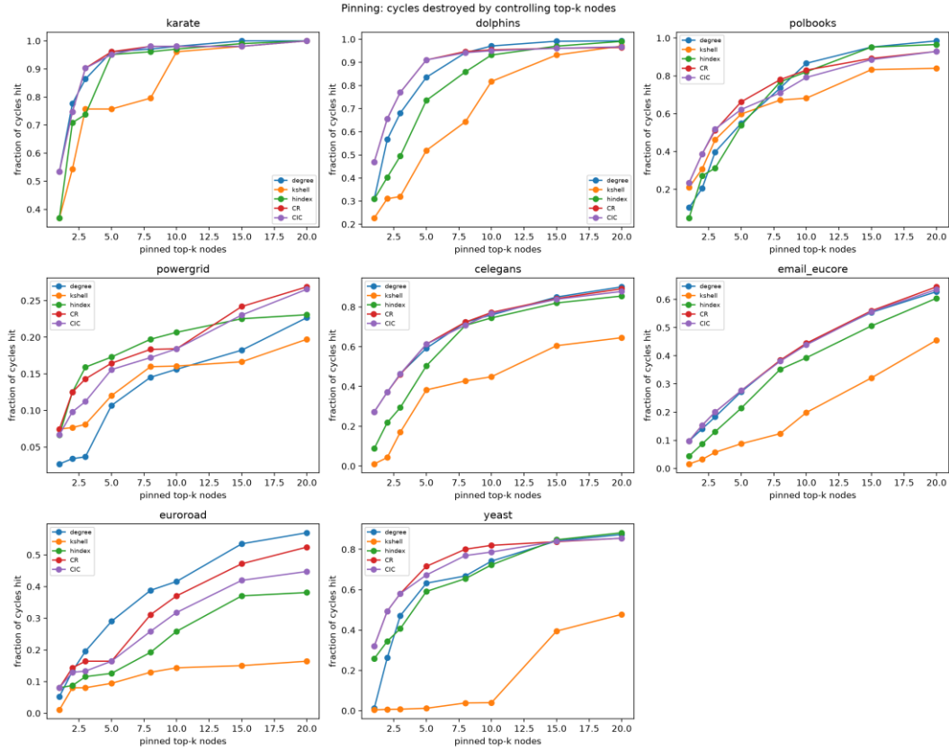
Figure 3. Fraction of cycles hit by pinning top- k nodes. CIC surpasses degree on the sparse power grid at all k \geq 5 , the cycle-native scenario for which CIC was designed.
