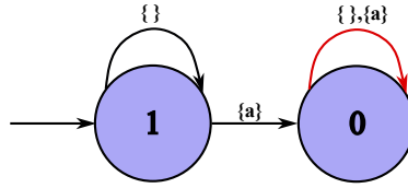
Figure 1: NBA representing the negated specification \mathbf{F}a . Accepting transitions (highlighted in red) are depicted as self-loops at state q_0 .
