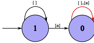
Figure 1: NBA representing the negated specification Fa . Accepting transitions (highlighted in red) are depicted as self-loops at state q_0 .
