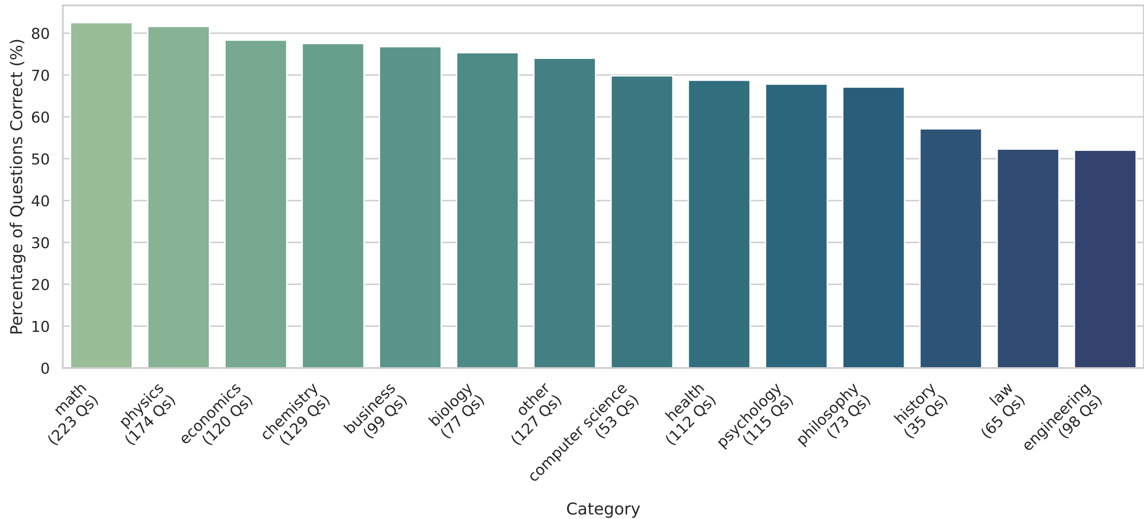
Category Accuracy (Majority Vote) (EVAL)
