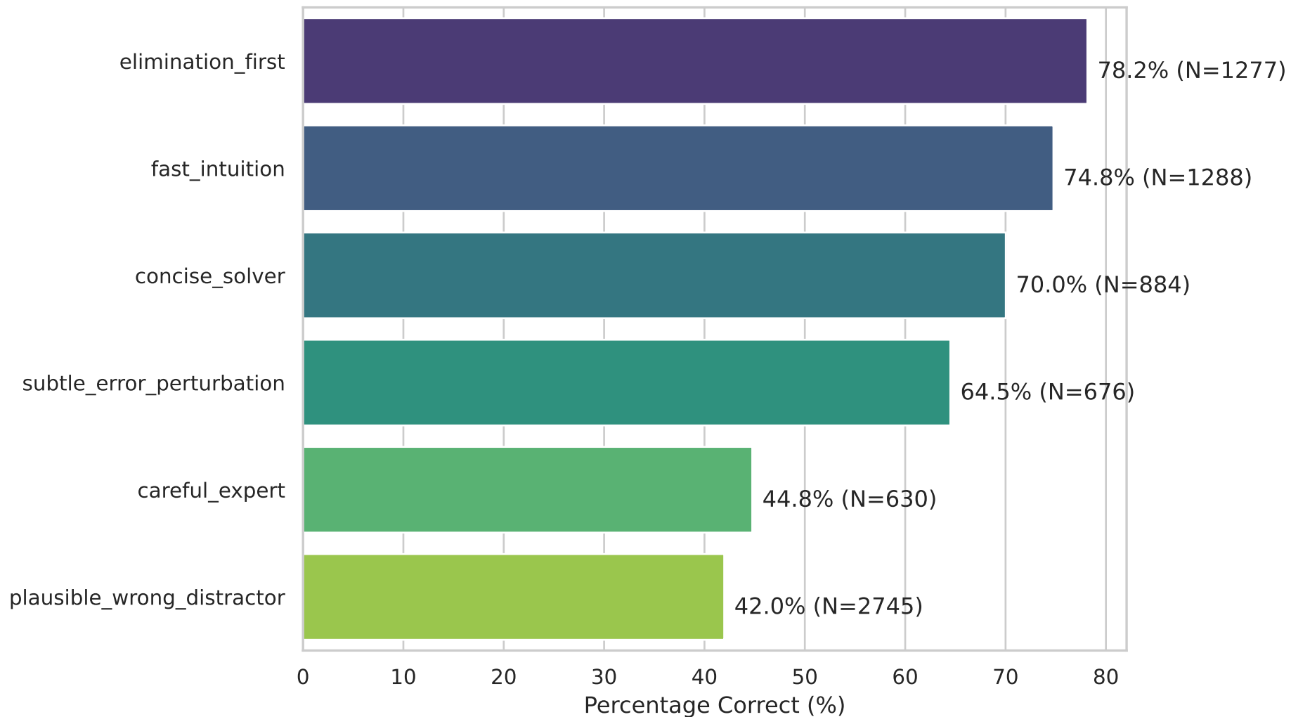
Trace-Level Accuracy by Expert Mode (EVAL)
