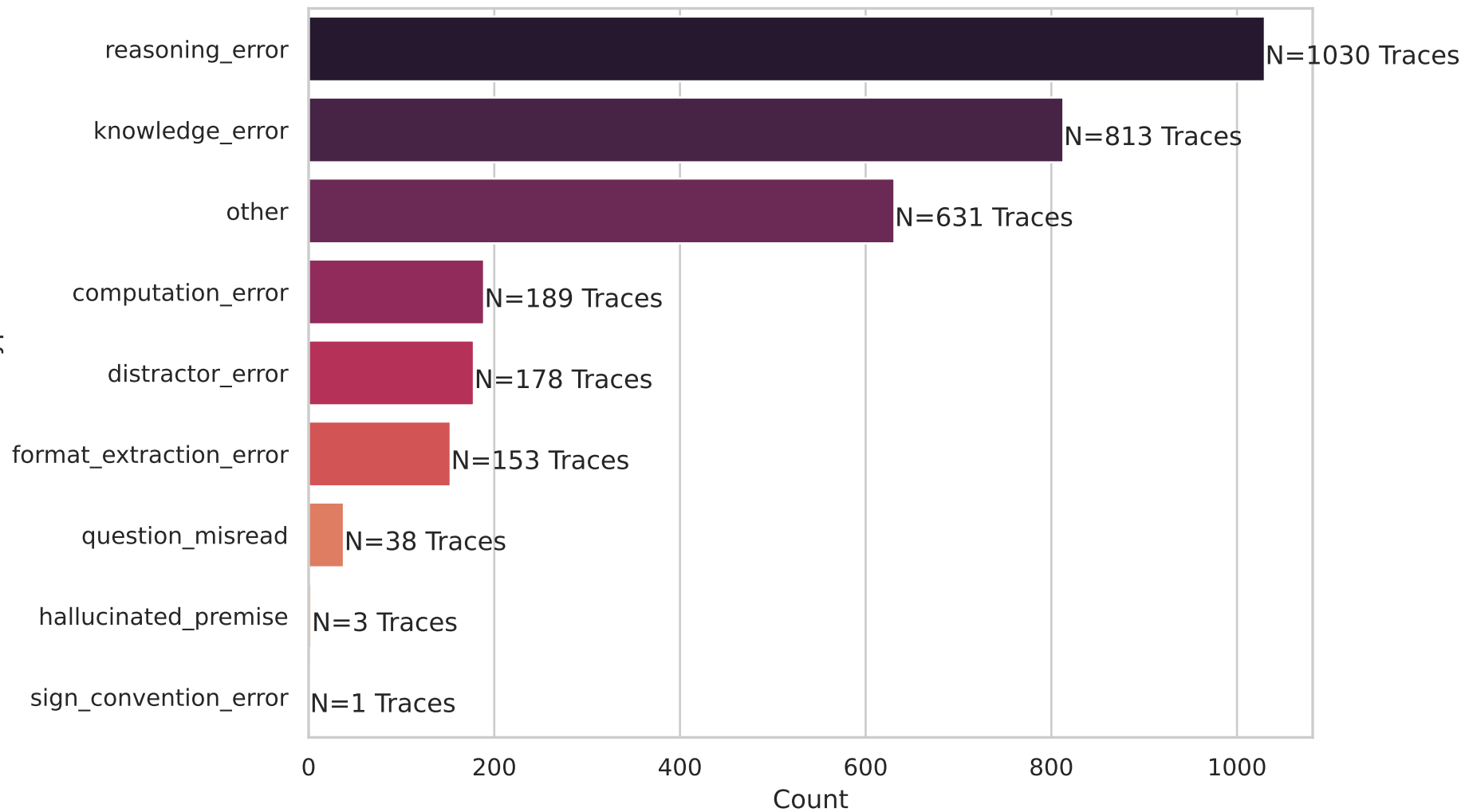
Distribution of Error Types (EVAL)
