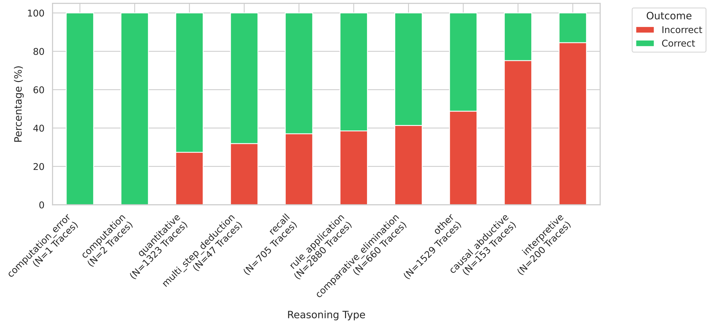
Correctness Rate by Dominant Reasoning Type (EVAL)
