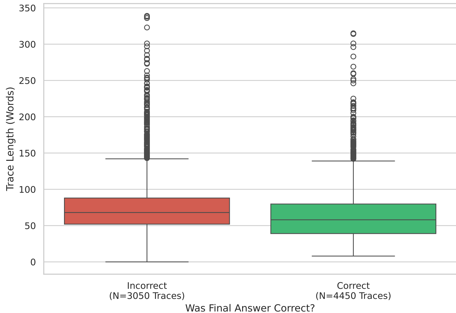
Trace Length vs. Outcome (EVAL)
