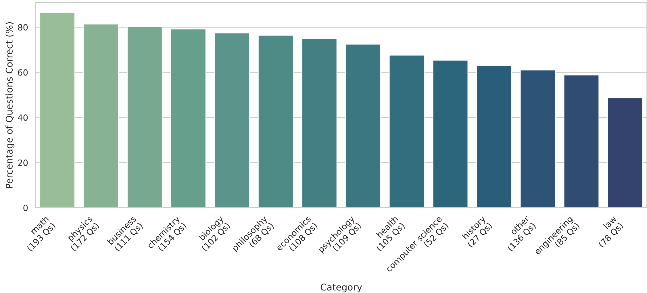
Category Accuracy (Majority Vote) (TEST)
