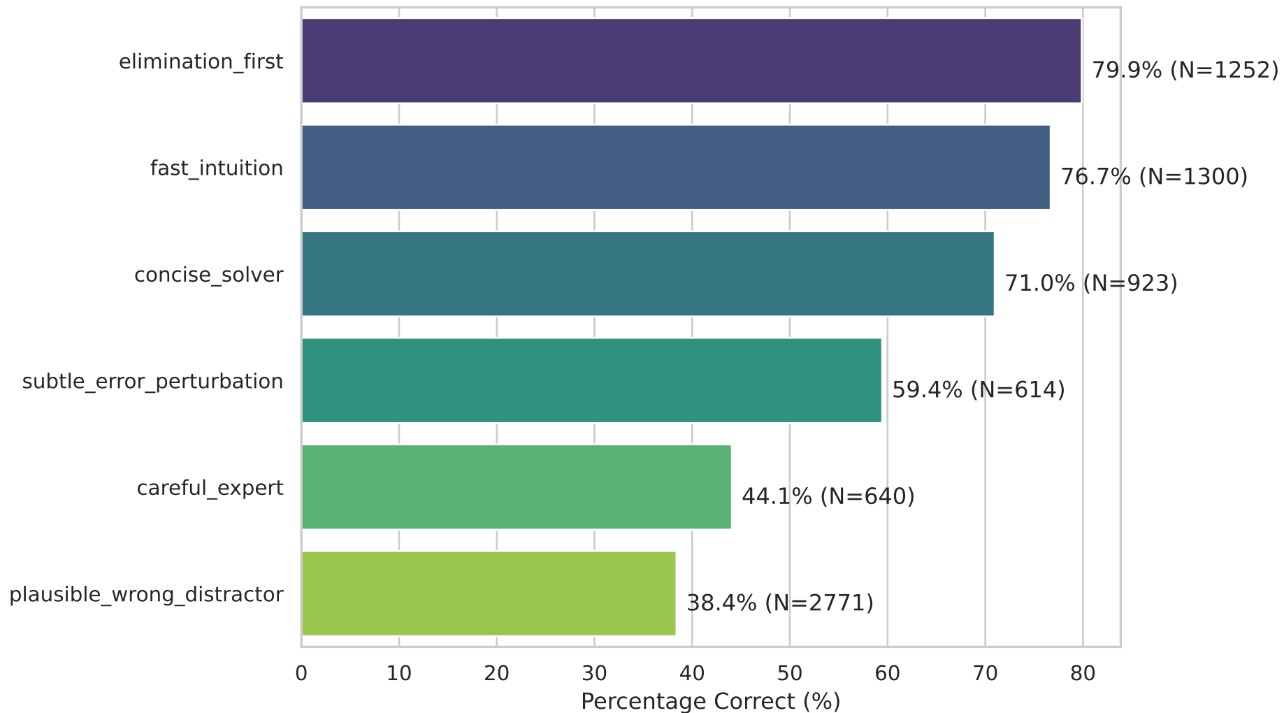
Trace-Level Accuracy by Expert Mode (TEST)
