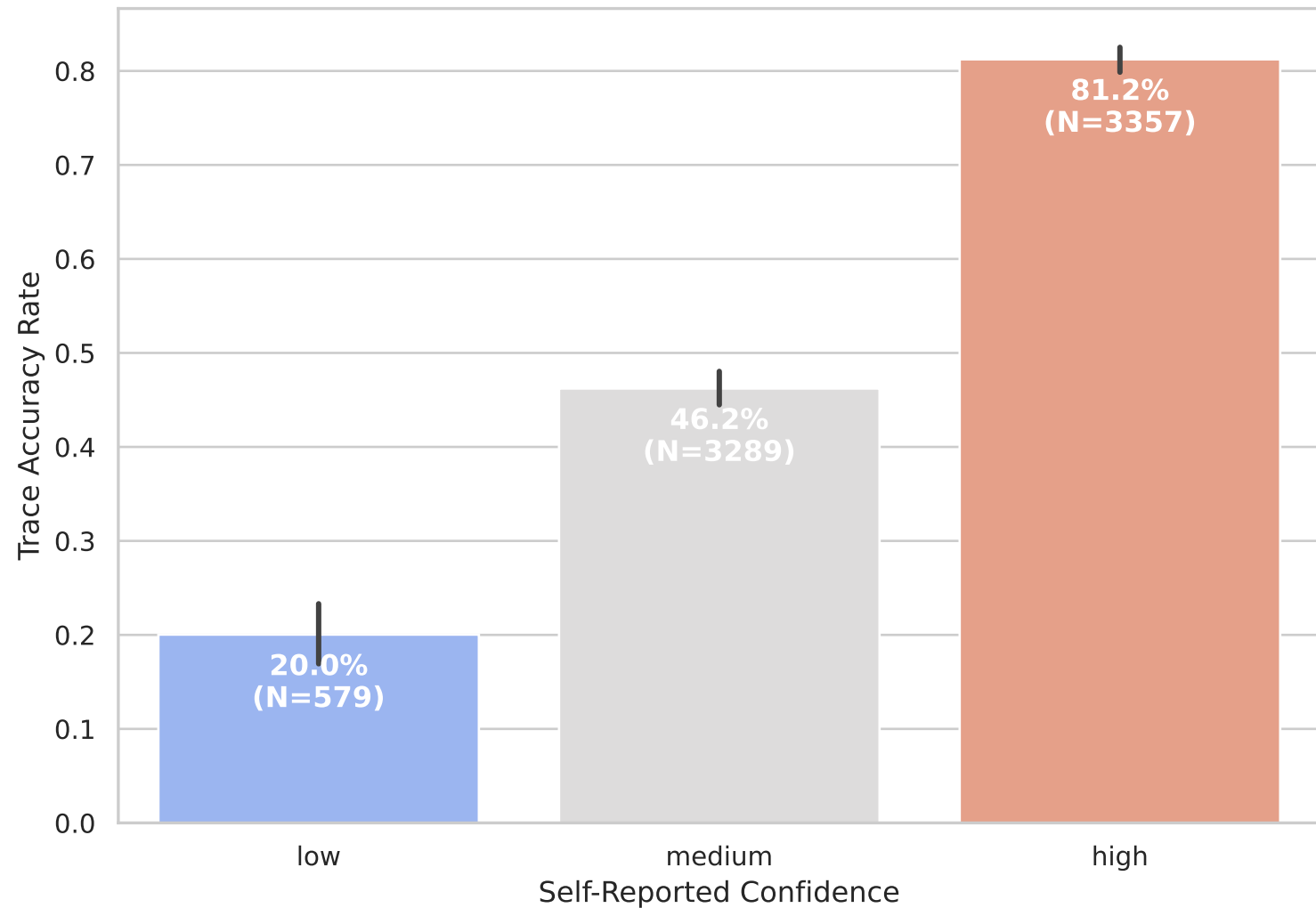
Uncertainty Calibration: Confidence vs. Trace Accuracy (TEST)
