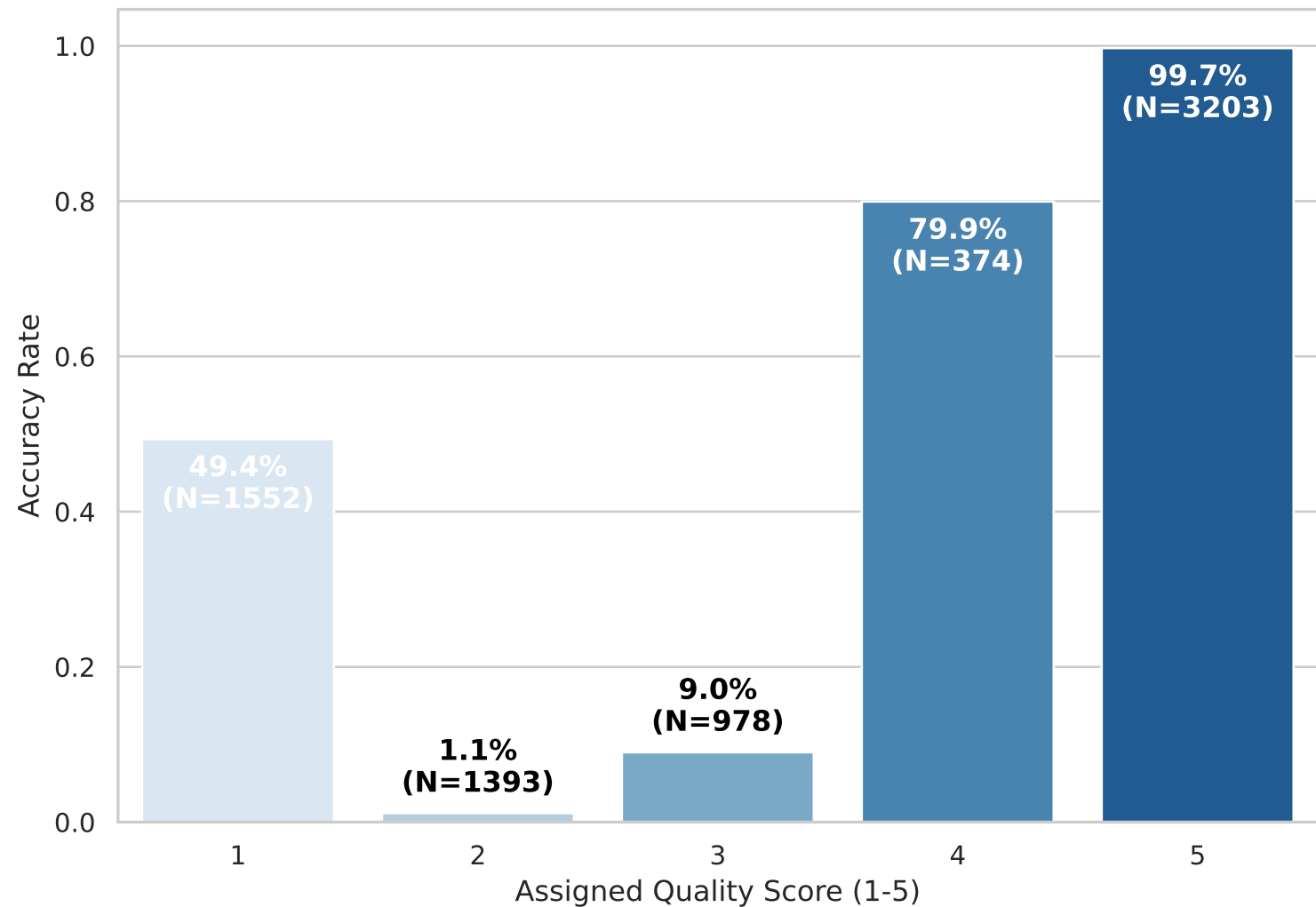
Annotator Quality Score vs. Trace Correctness (TEST)
