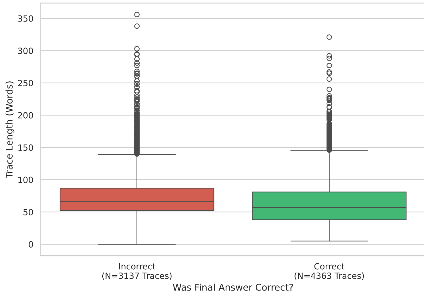
Trace Length vs. Outcome (TEST)
