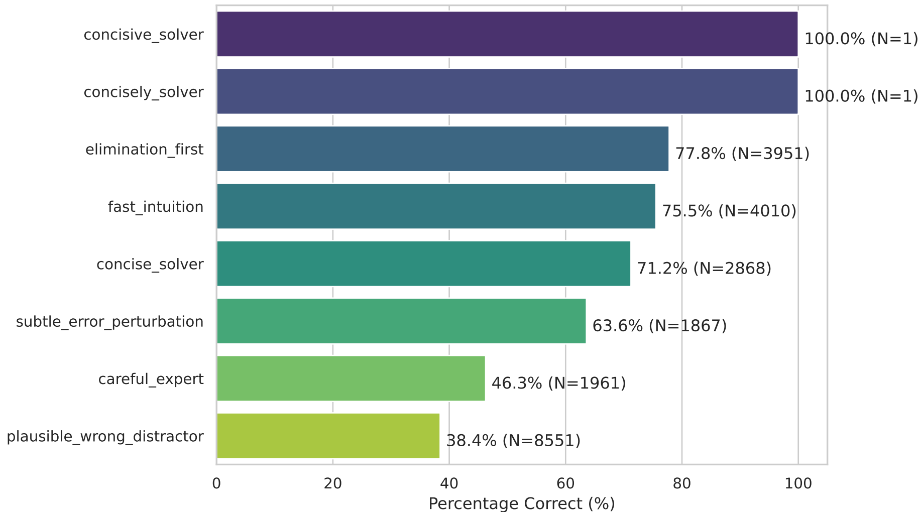
Trace-Level Accuracy by Expert Mode (TRAIN)
