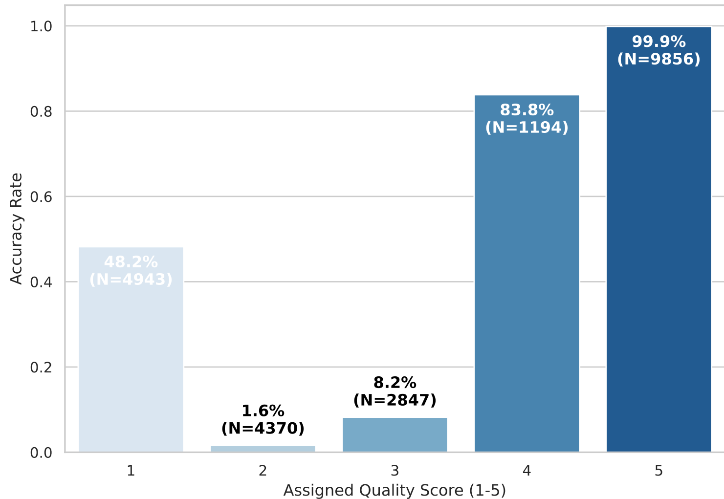
Annotator Quality Score vs. Trace Correctness (TRAIN)
