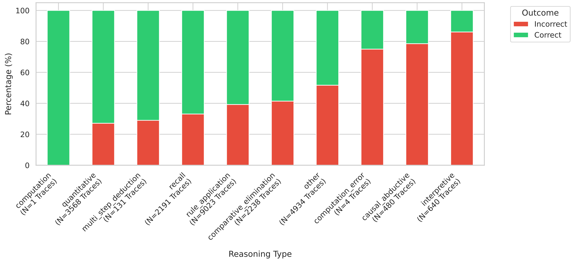
Correctness Rate by Dominant Reasoning Type (TRAIN)
