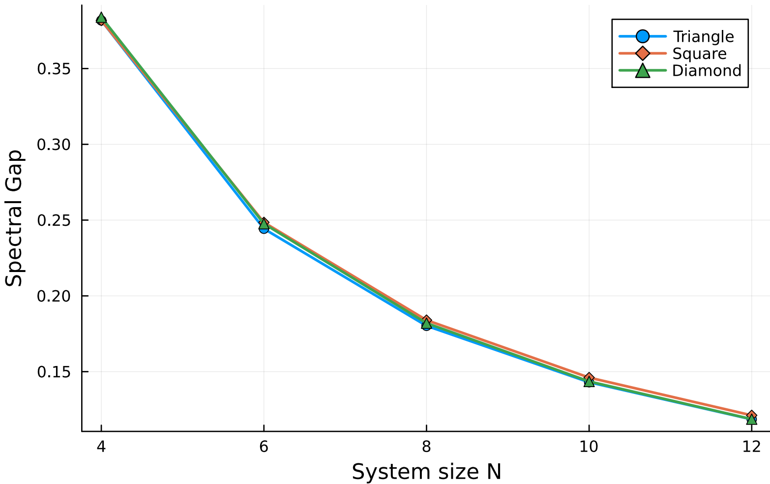
Gap vs N at \beta = 0.1
