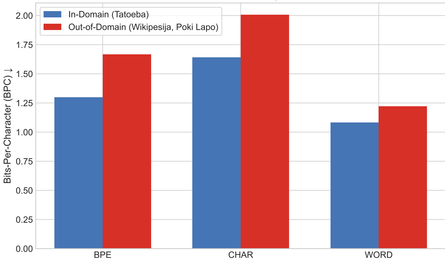
Pillar 1: Domain Generalization Gap across Tokenizers
