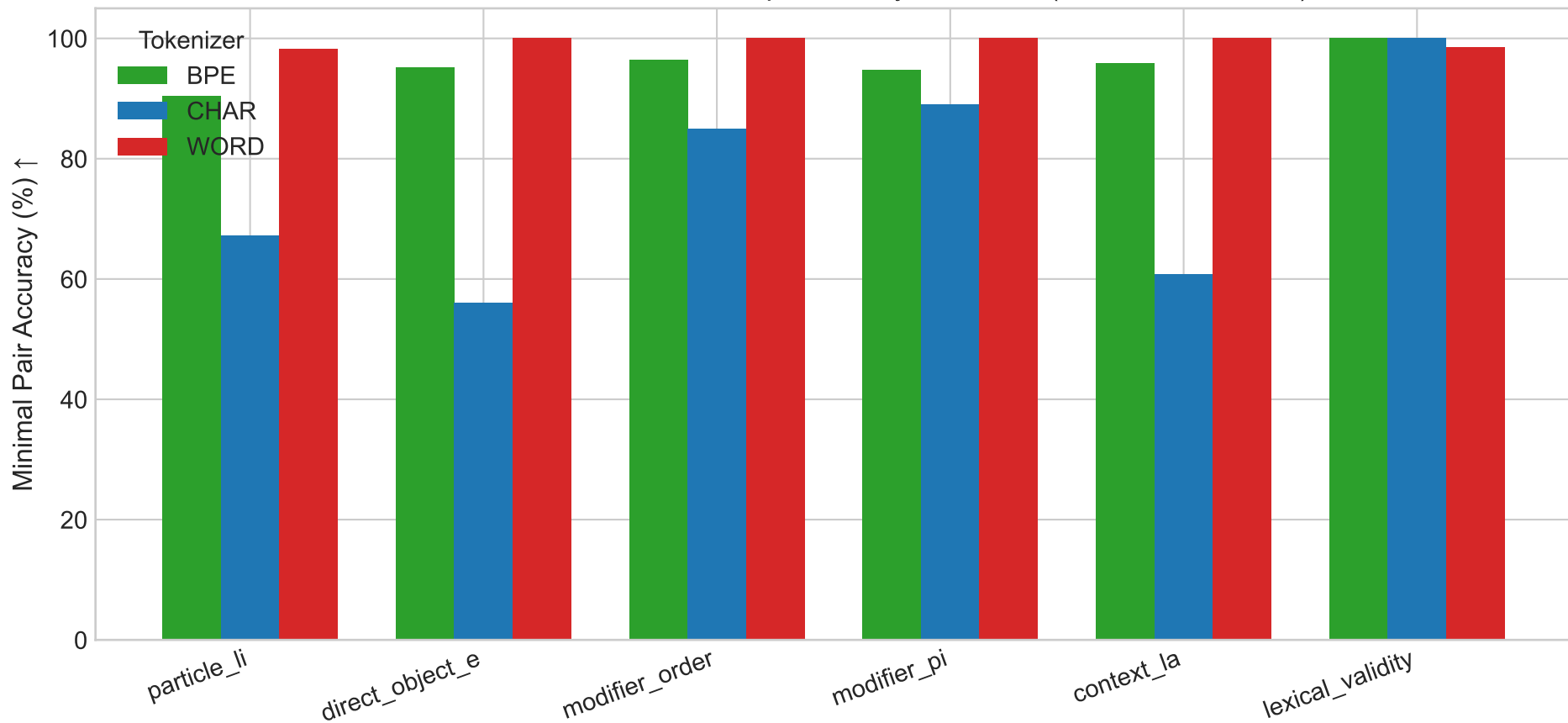
Pillar 2: Grammatical Rule Competence by Tokenizer (BLiMP Benchmark)
