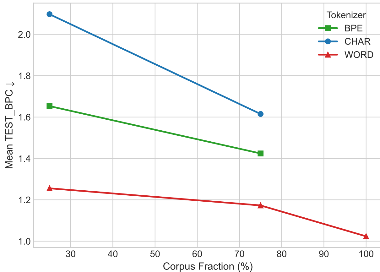
Interaction: Corpus Size × Tokenizer
