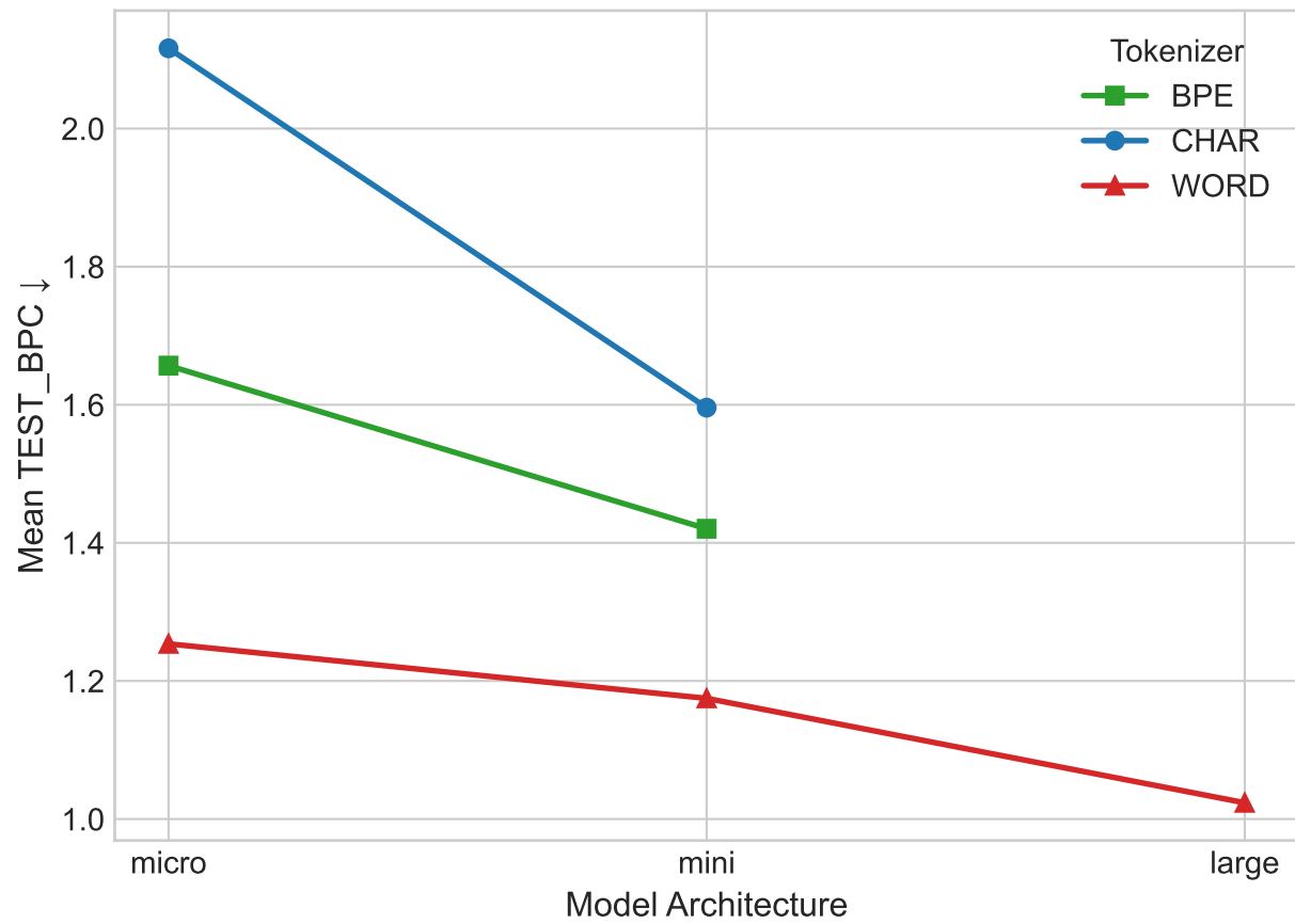
Interaction: Model Architecture × Tokenizer
