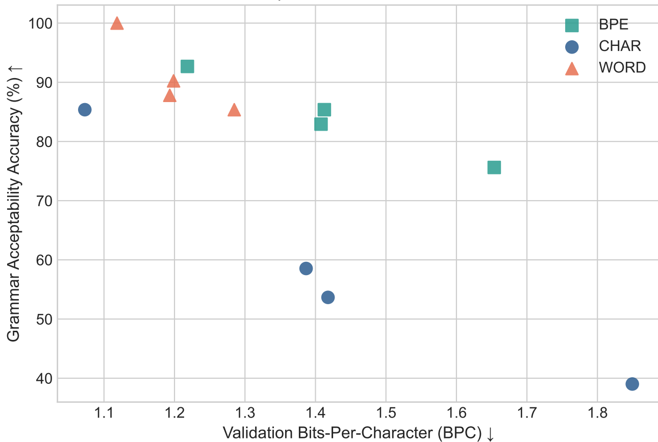
Grammatical Competence vs. Information-Theoretic BPC
