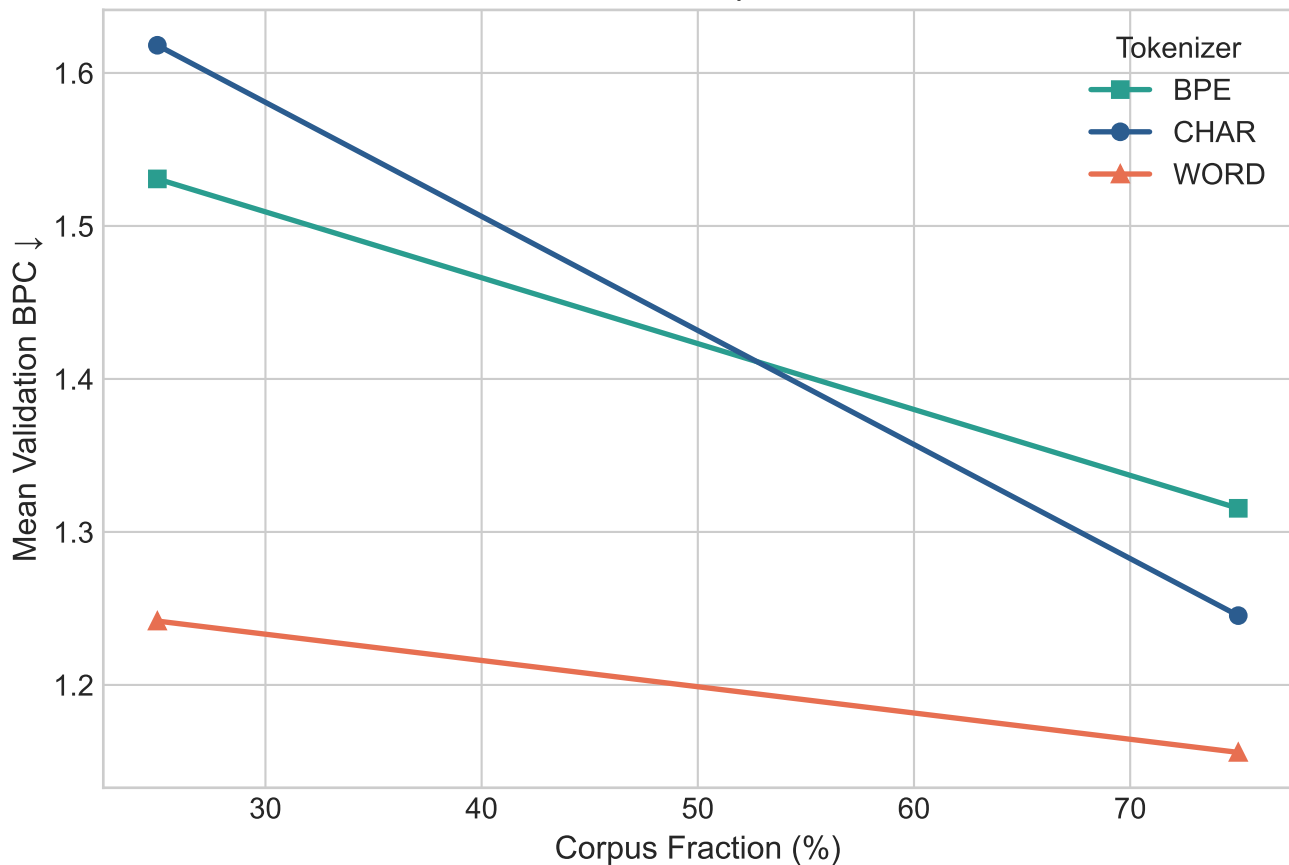
Statistical Interaction: Corpus Size × Tokenizer
