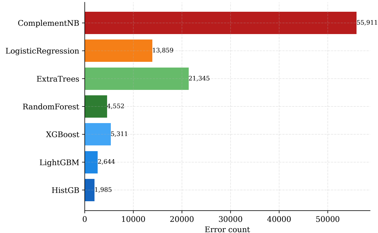
Misclassification Count — fold 0
