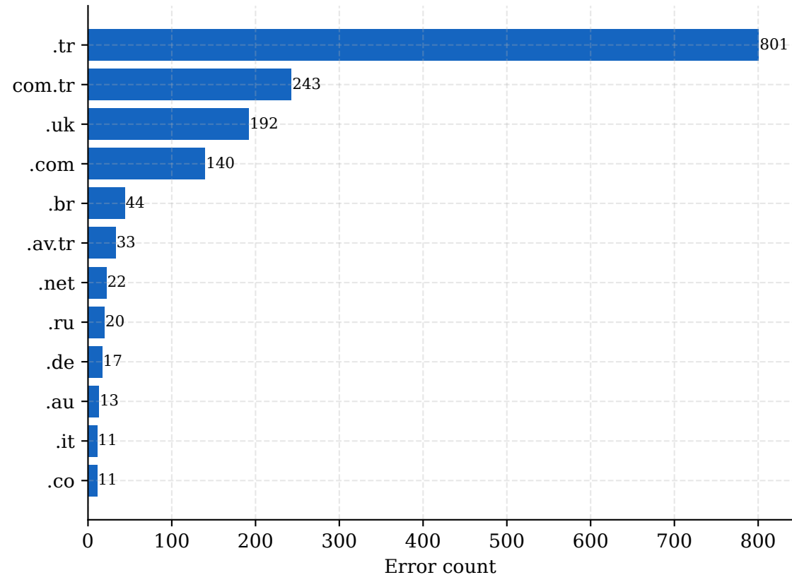
HistGB Errors by TLD — fold 0
