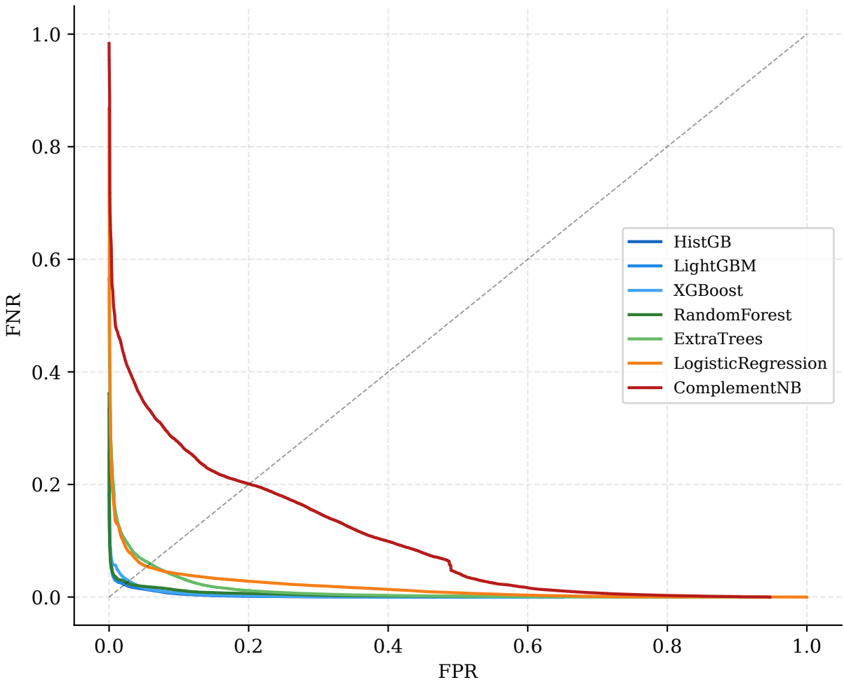
DET – fold 1
