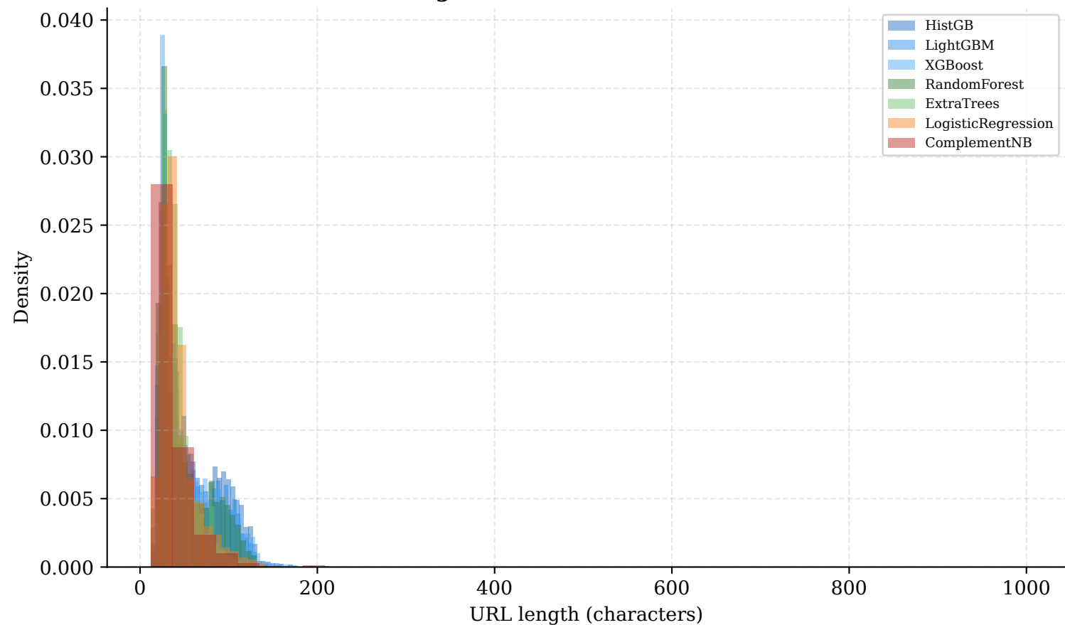
URL Length of Misclassified URLs — fold 1
